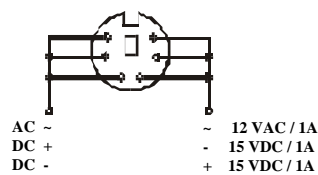
FIGURE 9: POWER SUPPLY CONNECTOR
