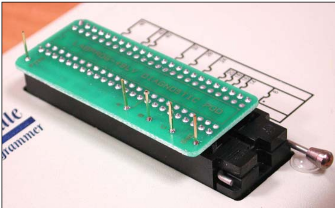
FIGURE 6: SELFTEST POD
