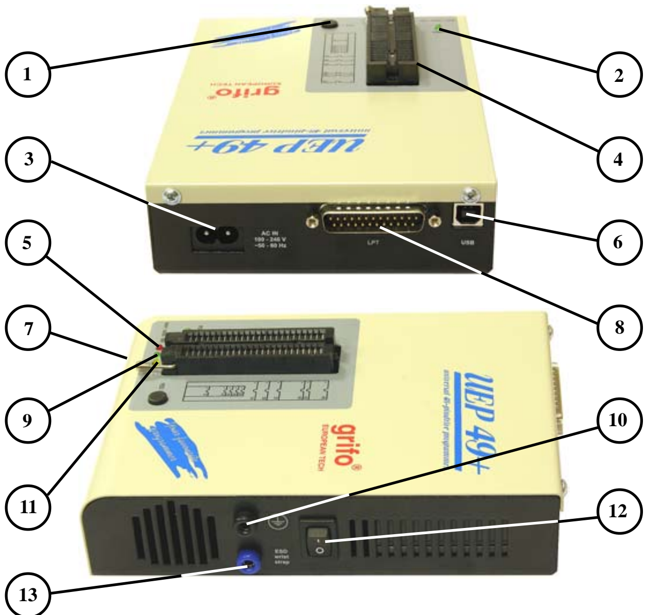
FIGURE 4: LEDs, CONNECTORS, BUTTON, ETC. LOCATION
