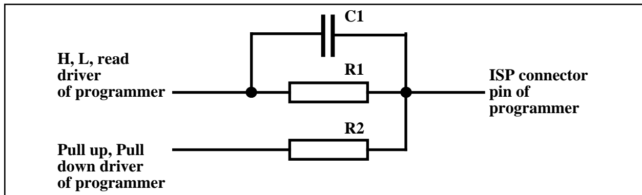
FIGURE 15: ISP SIGNALS CONNECTION ON PROGRAMMER
