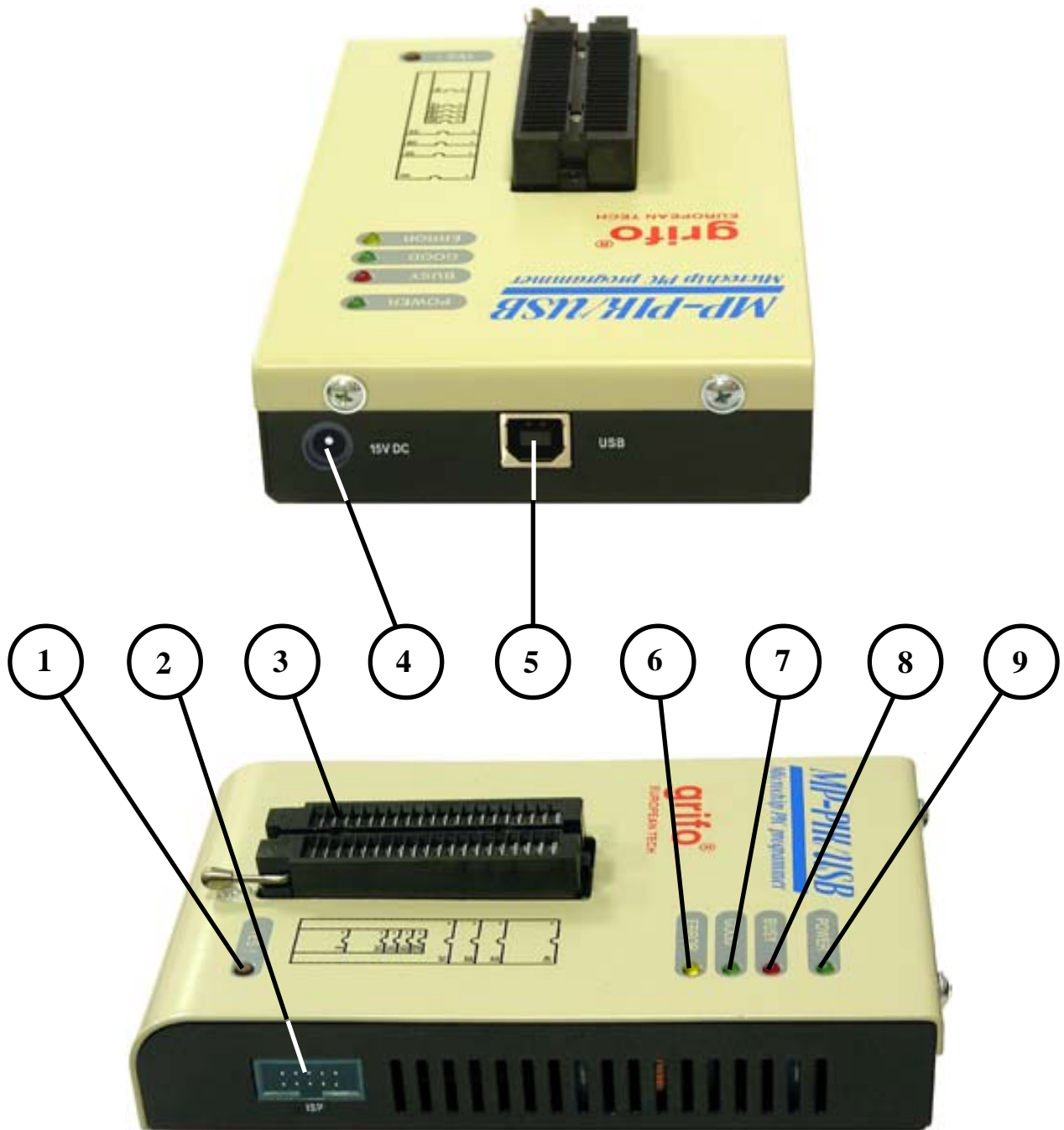
FIGURE 4: LEDs, CONNECTORS, BUTTON, ETC. LOCATION
