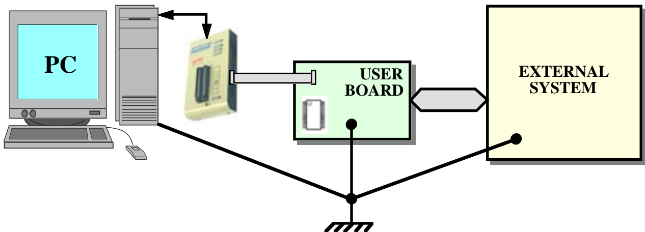
FIGURE 12: CONNECTION FOR ISP PROGRAMMING
