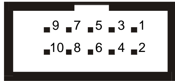
FIGURE 13: ISP CONNECTOR
