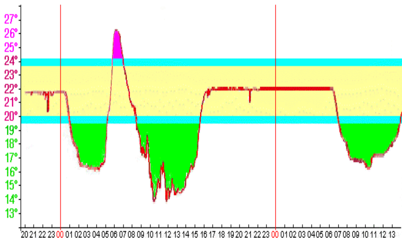
Temperature control profile on a time base.
