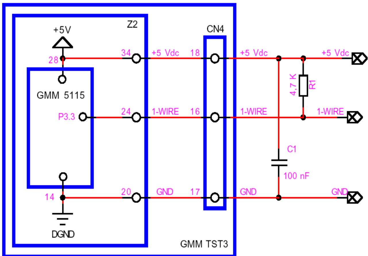
1-Wire interfacement circuit.
